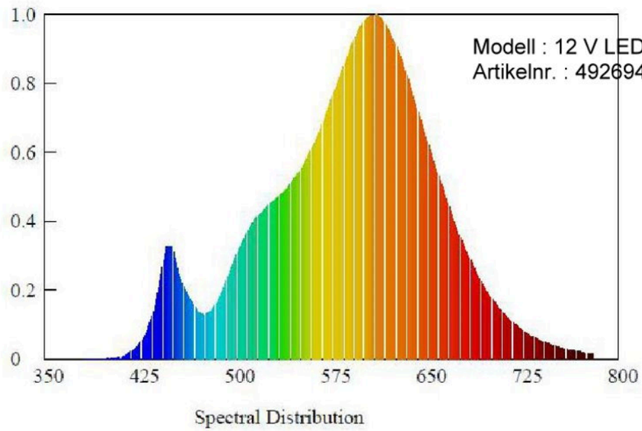
Spectral power distribution (2700K)
